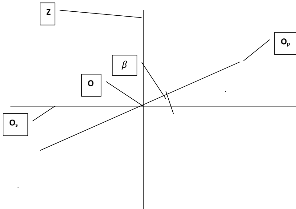
Pic. 1 Cross section of the solar system.
